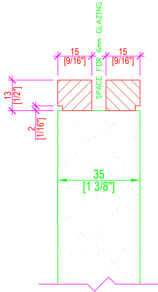
FLUSH GLAZING STOP 1-3/8" (35mm) DOOR SCALE: 1:1
