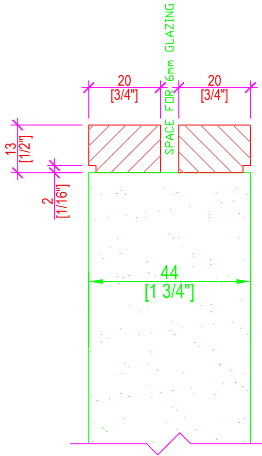
FLUSH GLAZING STOP 1-3/4" (44mm) DOOR SCALE: 1:1
